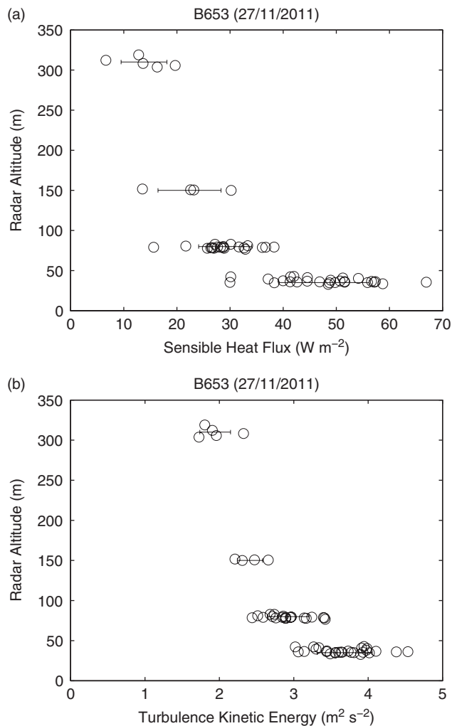
Figure 8. Profiles of (a) sensible heat flux and (b) turbulent kinetic energy for flight B653 (27 November 2011). Circles show run averages, horizontal lines show the mean and standard deviation for each altitude range.
