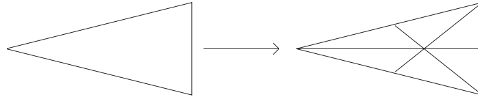
FIGURE 6.17. Barycentric subdivision
