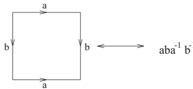
FIGURE 6.1. The torus as an identification space
