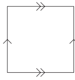
FIGURE 1.5. The torus
