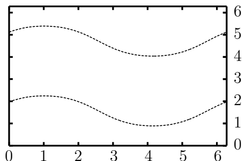
FIGURE 7. \mathbf{N}_1^\nu(\alpha) for Example 5.2.
