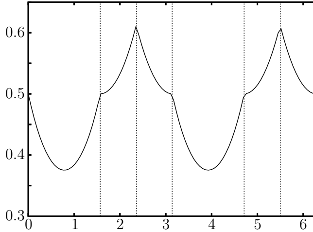
FIGURE 4. \bar{\Omega}_\alpha for Ledrappier's example.
