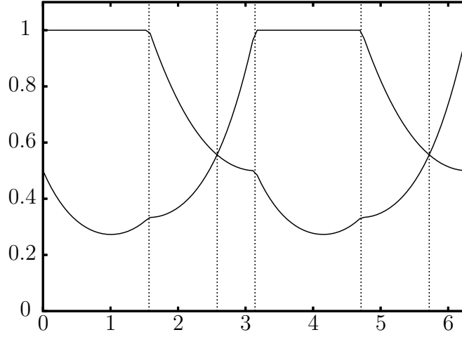
FIGURE 3. \bar{\Omega}_\alpha for the \times 2, \times 3 system in Example 4.1.
