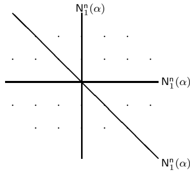
FIGURE 2. The three non-expansive lines for Ledrappier’s example.
