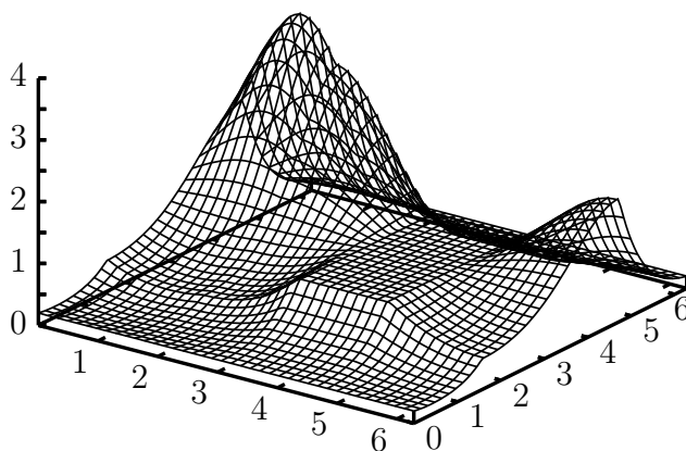
FIGURE 6. A layer of \bar{\Omega}_\alpha for Example 5.2.
