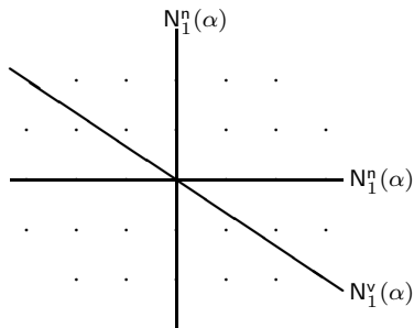
FIGURE 1. The three non-expansive lines for \times 2, \times 3 .
