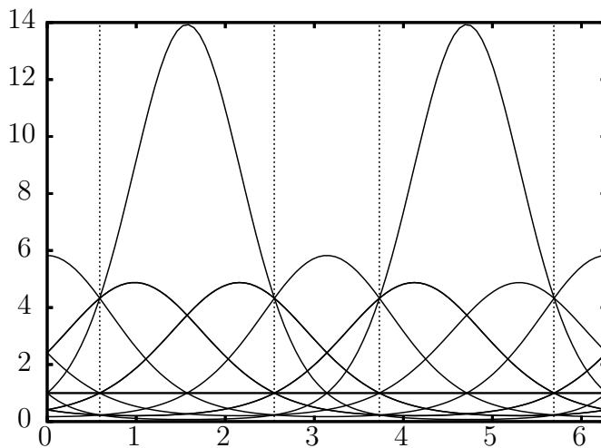
FIGURE 5. \bar{\Omega}_\alpha for Example 5.1.
